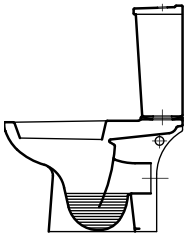
Close coupled wc suite W 36.1cm D 61cm H 79cm
