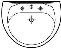
56cm semi-recessed basin W 55.2cm D 49.8cm H 18.6cm
